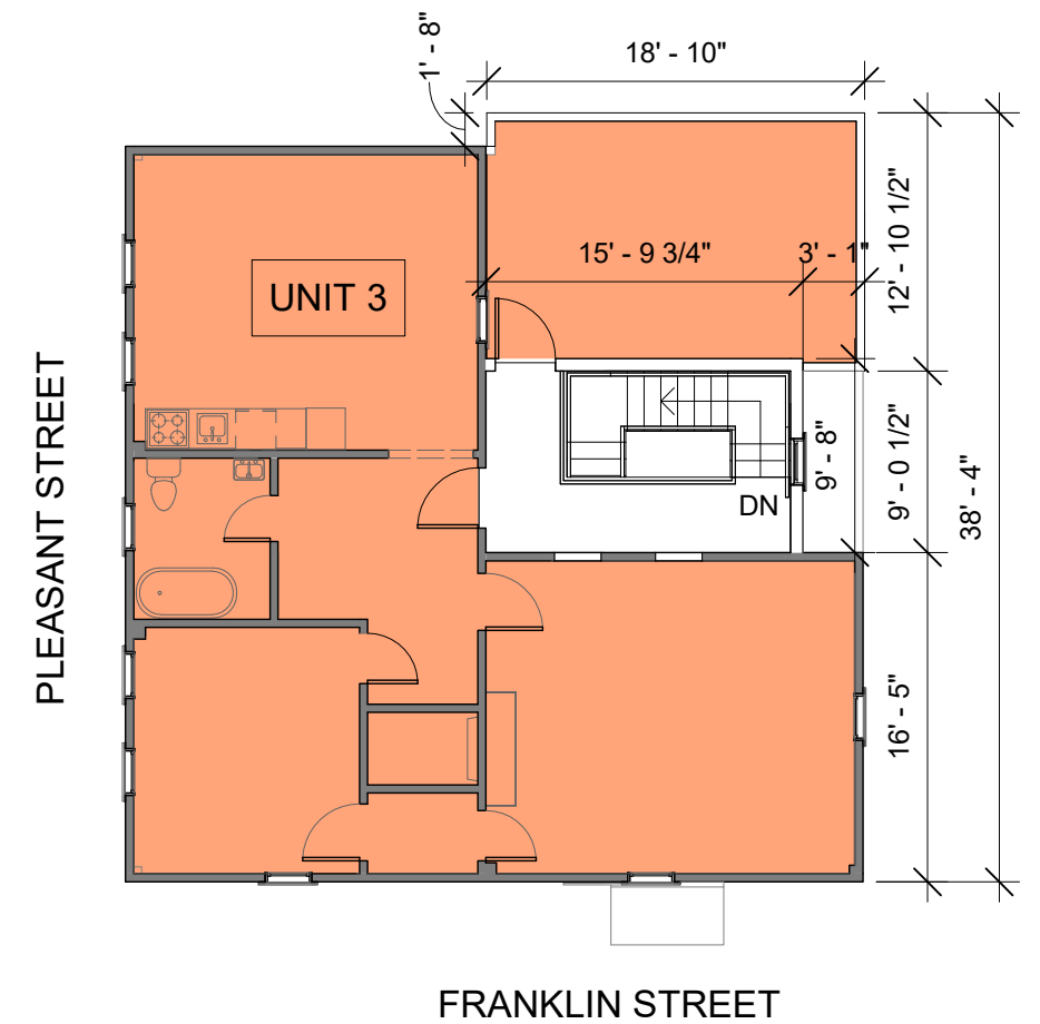
3 THIRD FLOOR 3/32" = 1'-0"
