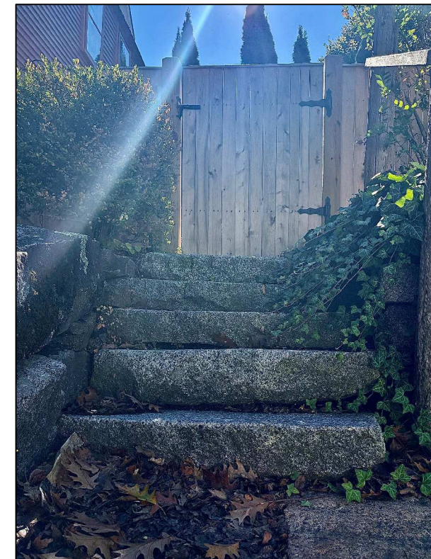
Close Up of Landscape Steps Irregular, steep rise and shallow run dimensions
