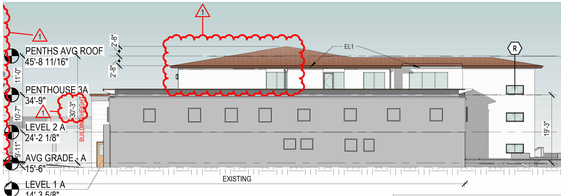
1 NORTH ELEVATION
