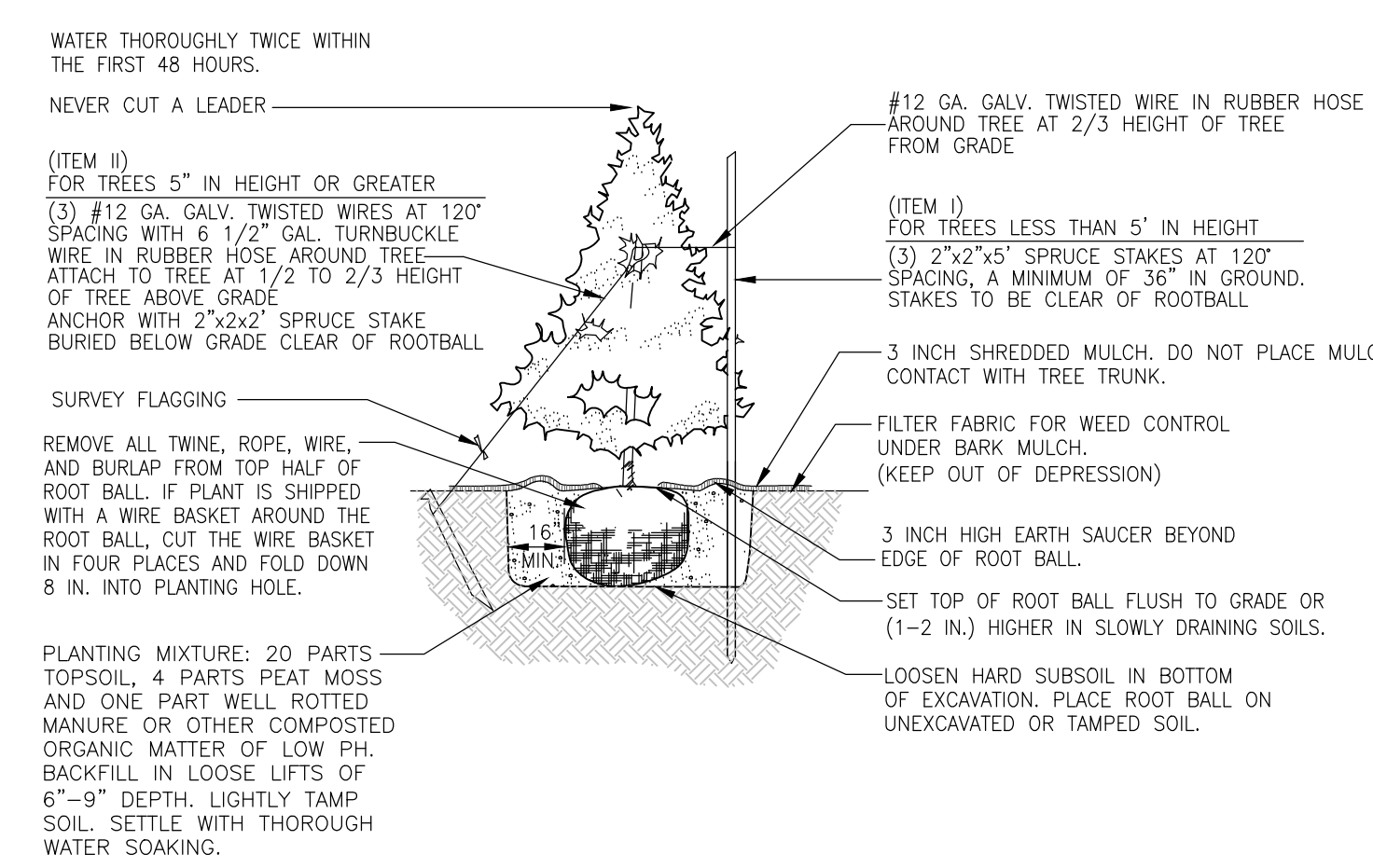
EVERGREEN PLANTING NOT TO SCALE
