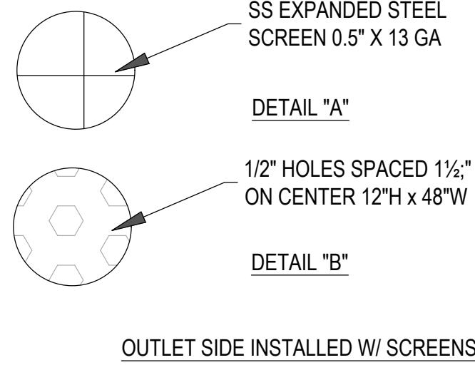
OUTLET SIDE INSTALLED W/ SCREENS
