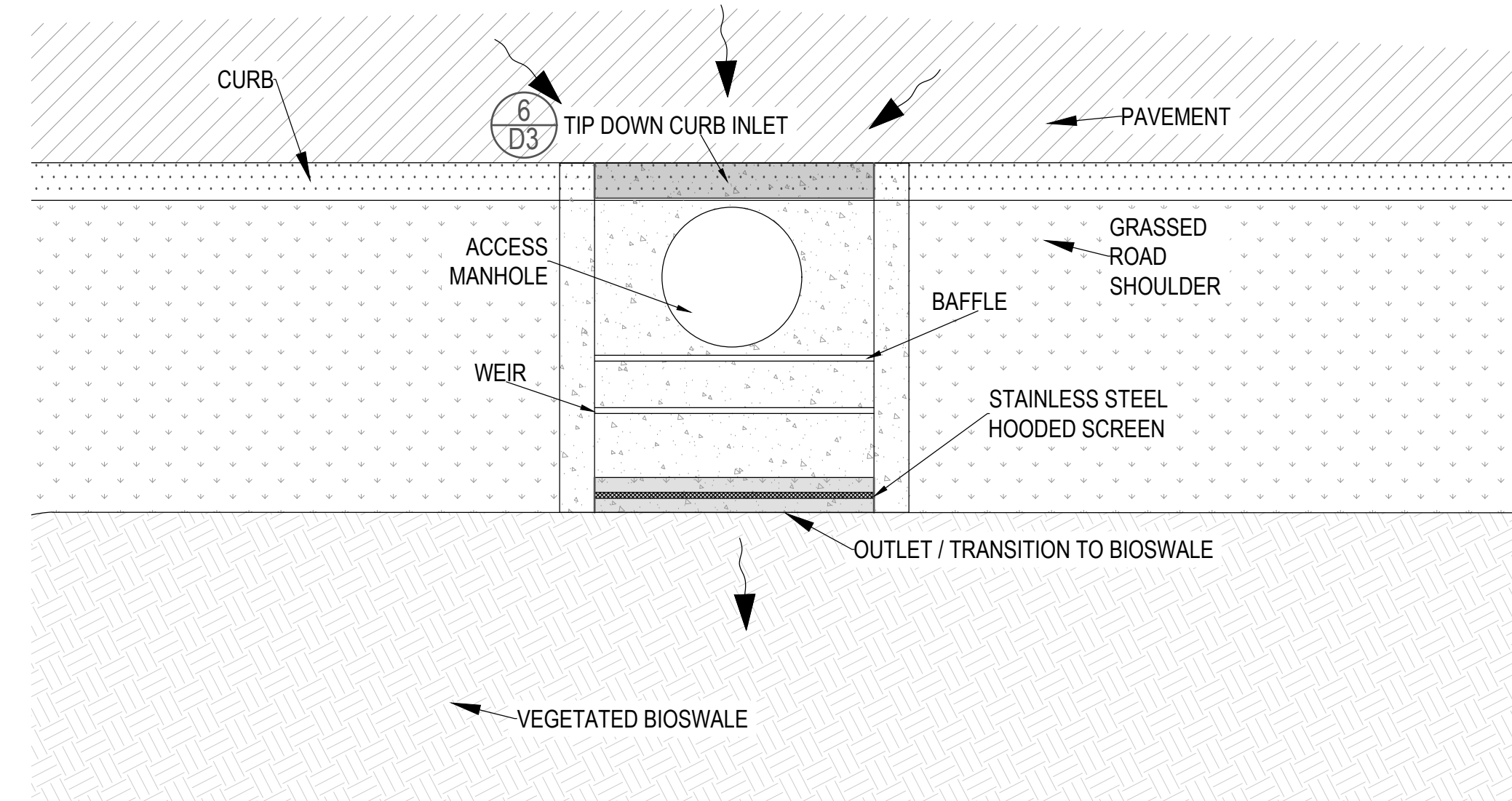
7 PRETX CURB OUTLET TO BIORETENTION CONFIGURATION
