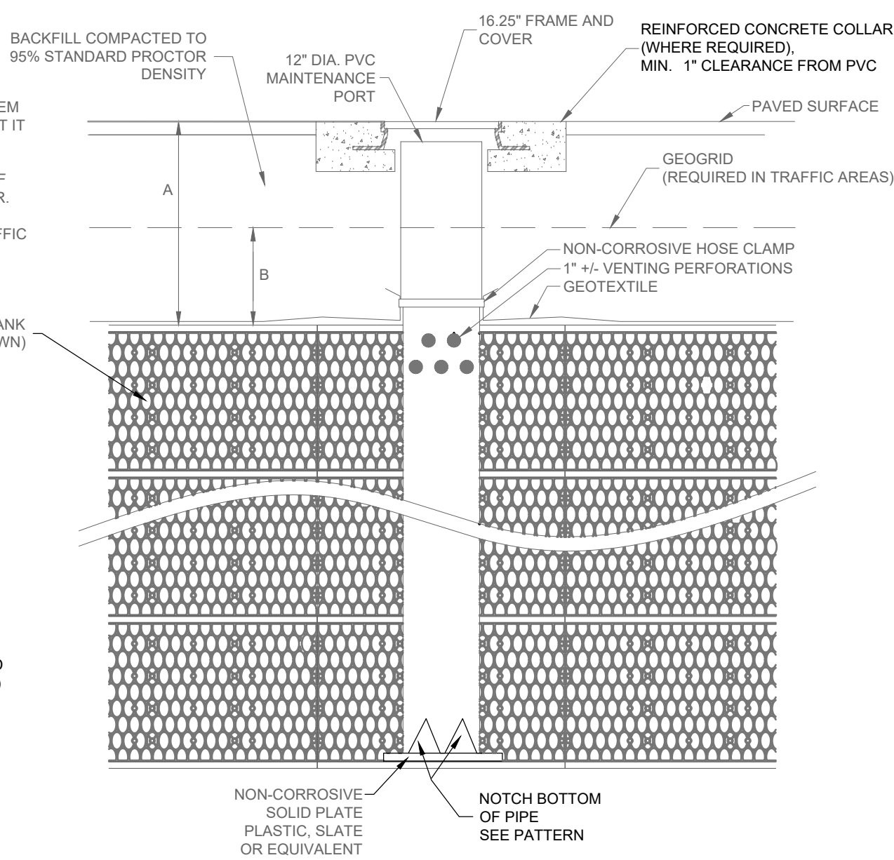
MAINTENANCE PORT FOR R-TANK SD , R-TANK HD , AND R-TANK SD
