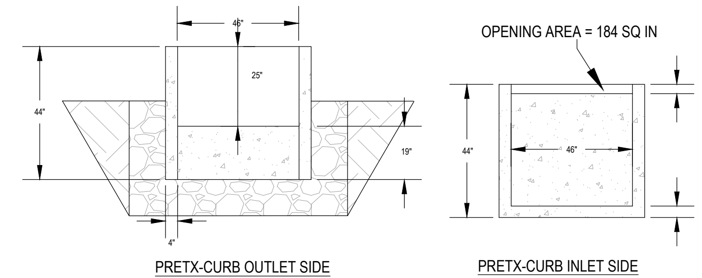
4 PRETX CURB SIDE DETAIL NOT TO SCALE
