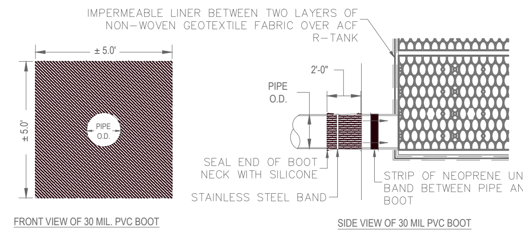
R-TANK TYPICAL INLET/OUTLET W/ 30 MIL PVC BOOT
