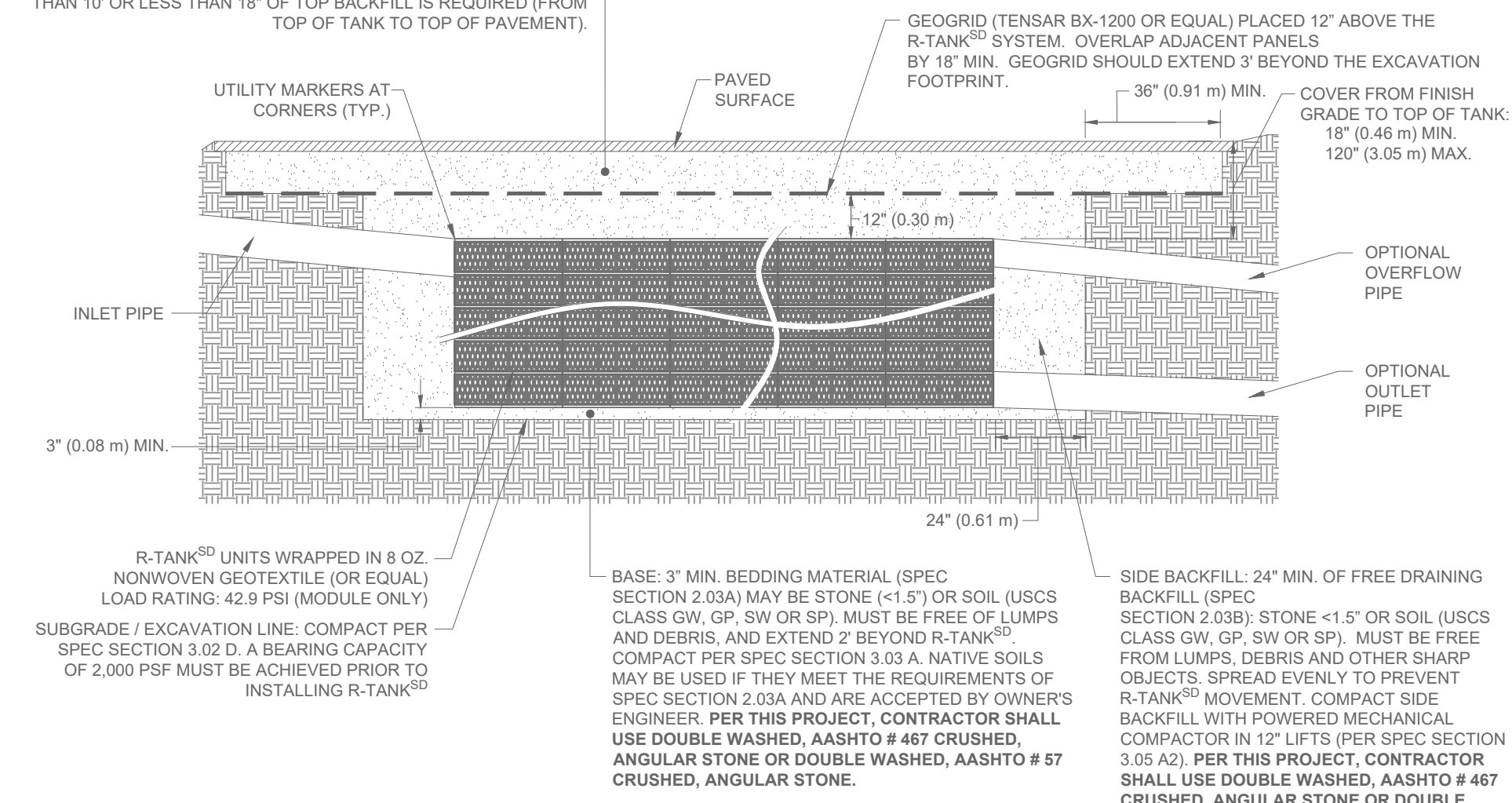
R-TANK SD & HS-20 LOADS - SECTION VIEW
