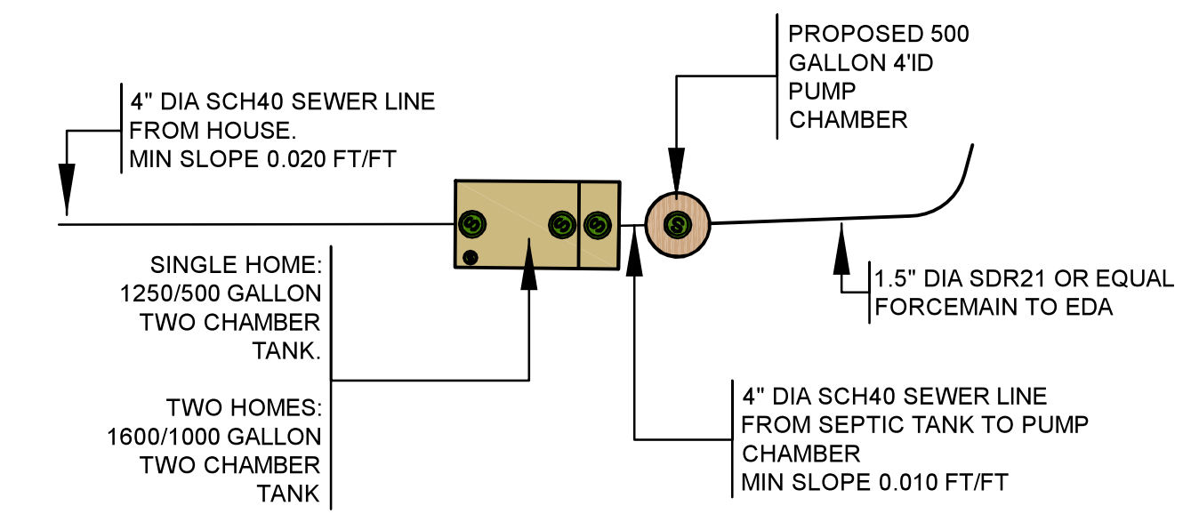
SEPTIC TANK AND PUMP CHAMBER LAYOUT (TYP)
