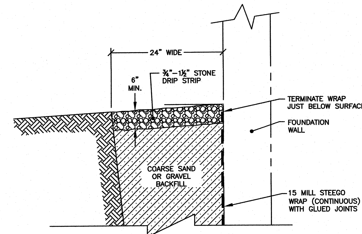
C STONE DRIP APRON SEE ARCHITECT'S PLAN FOR NTS DETAIL AT NEW FOUNDATION
