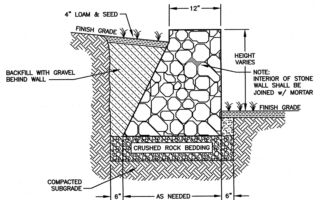
B STONE WALL DETAIL NTS
