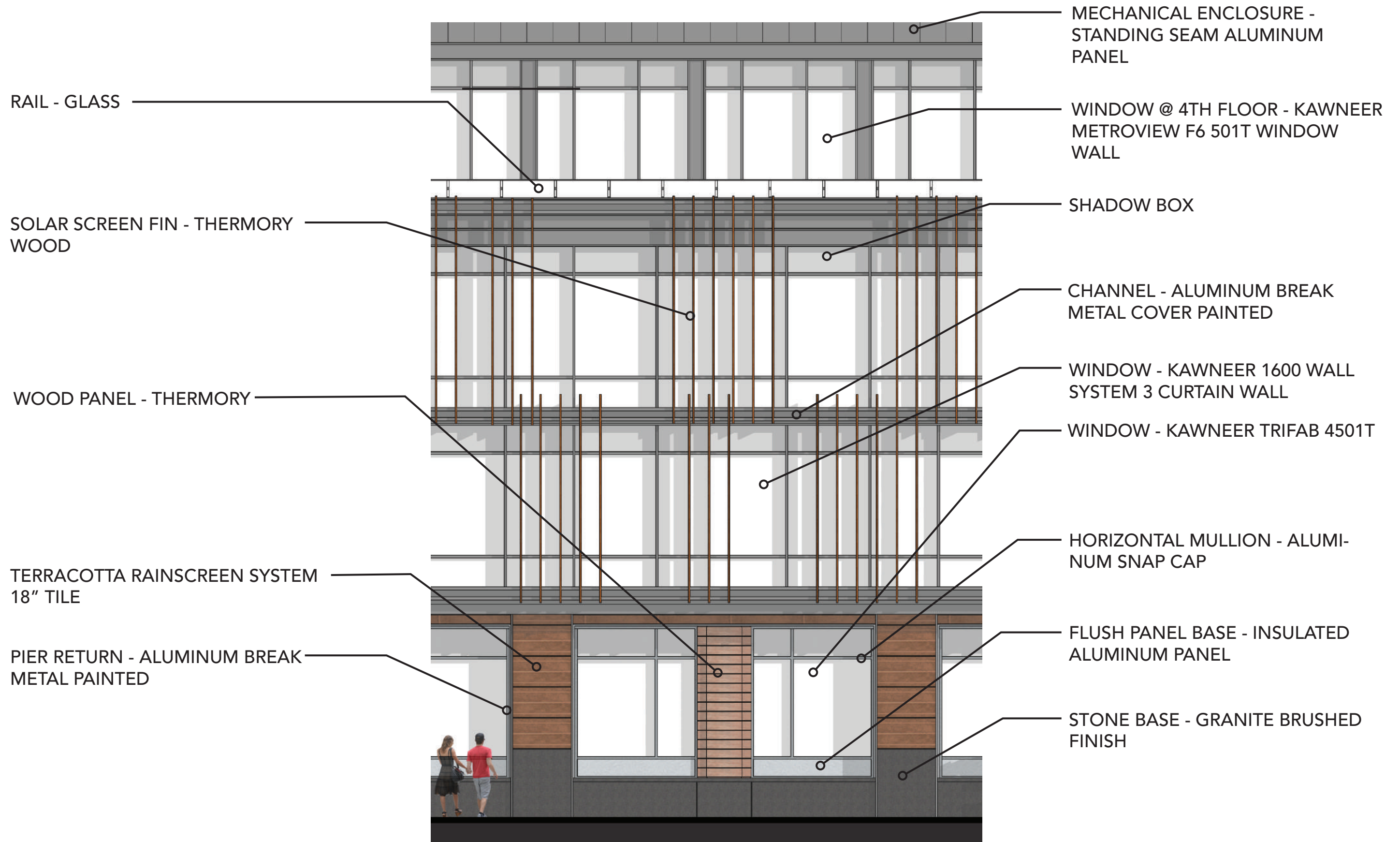
Typical Bay - Raynes Projection
