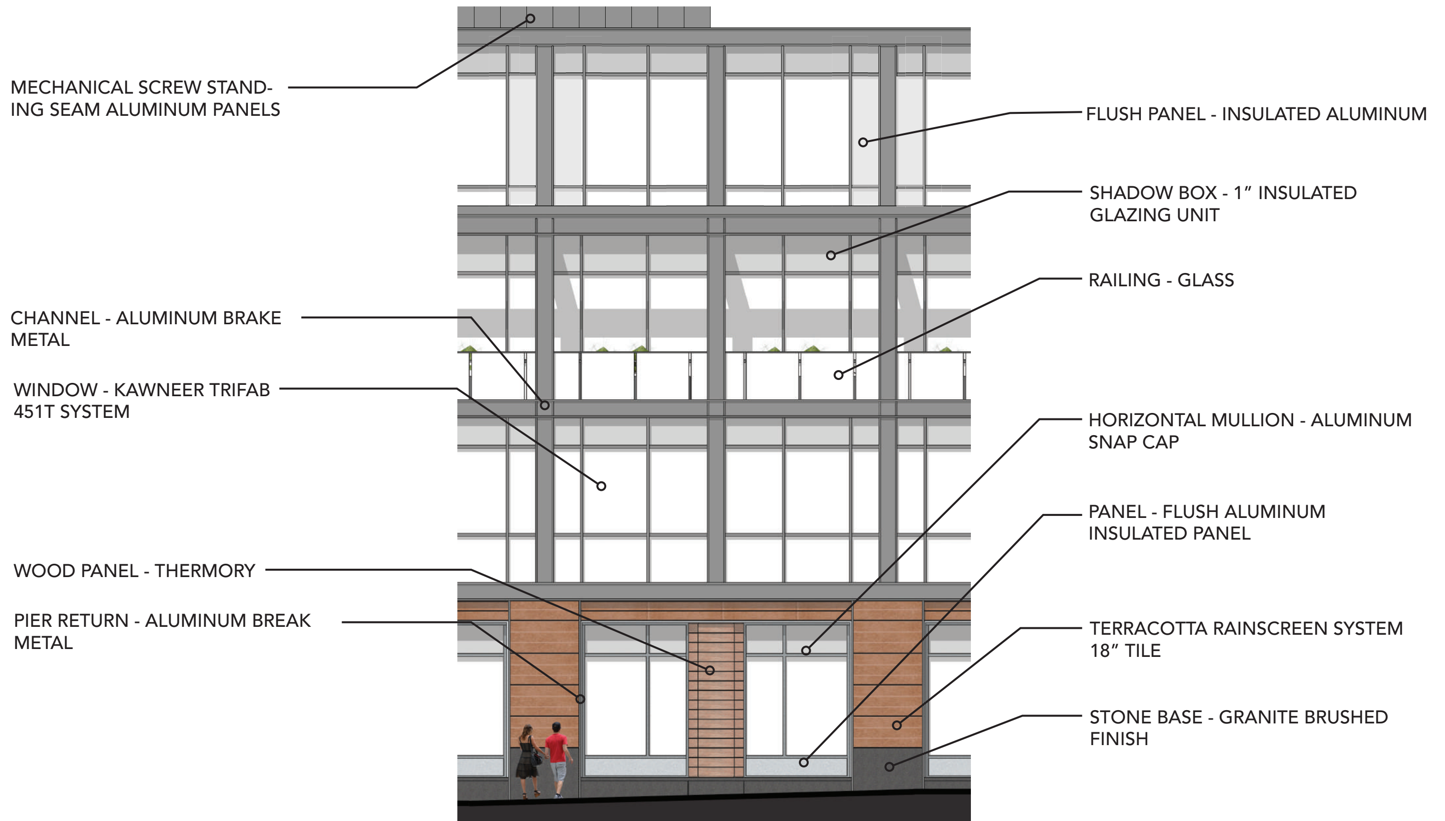
Typical Bay - Veranda
