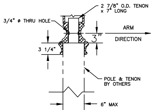
TENON DETAIL
