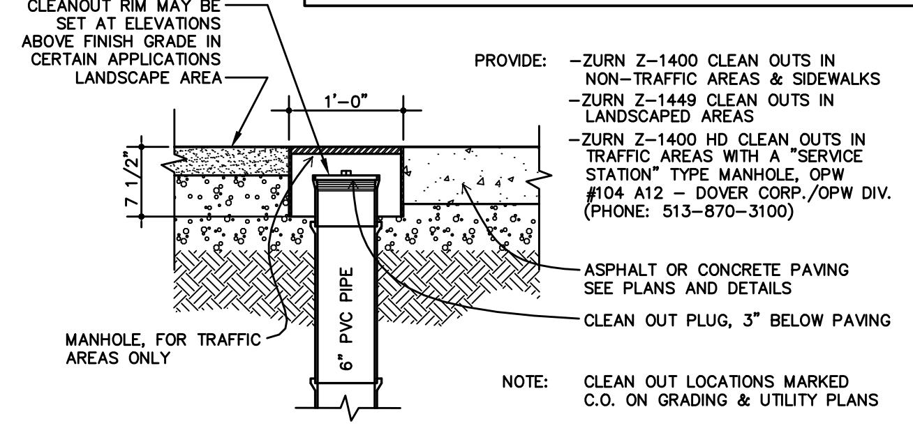
CLEANOUT NOT TO SCALE
