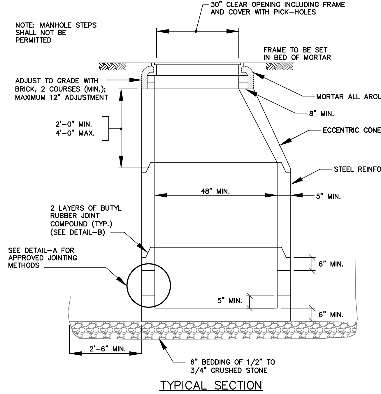
SEWER MANHOLE NOT TO SCALE
