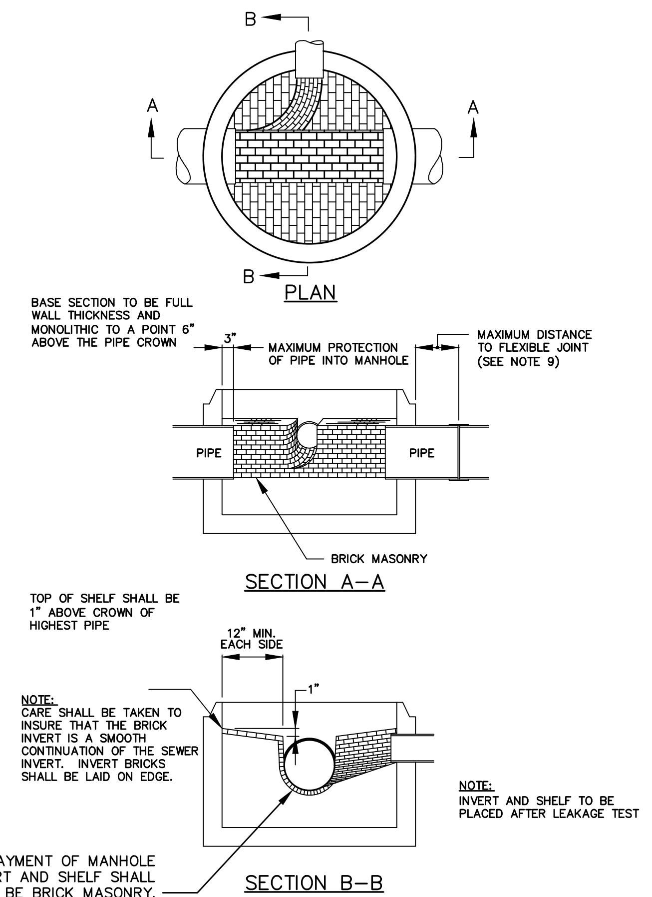
SEWER MANHOLE NOT TO SCALE
