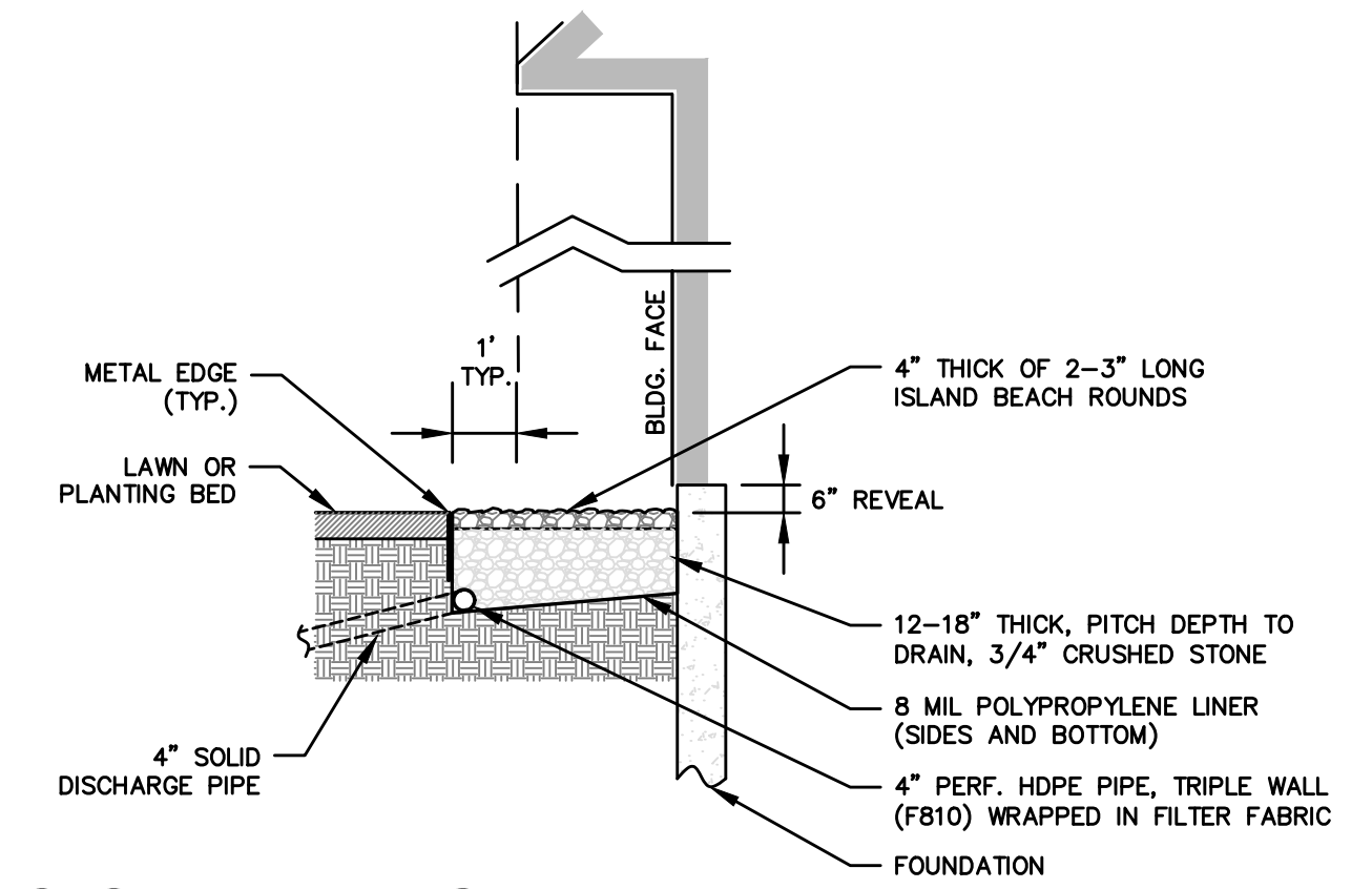
STONE DRIP EDGE NOT TO SCALE
