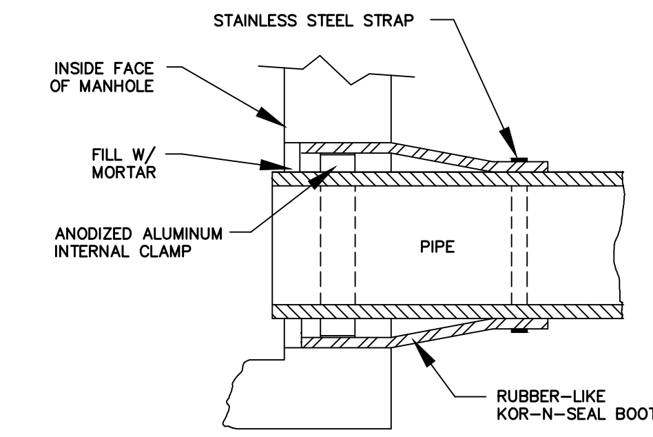
SEWER MANHOLE DETAIL A NOT TO SCALE
