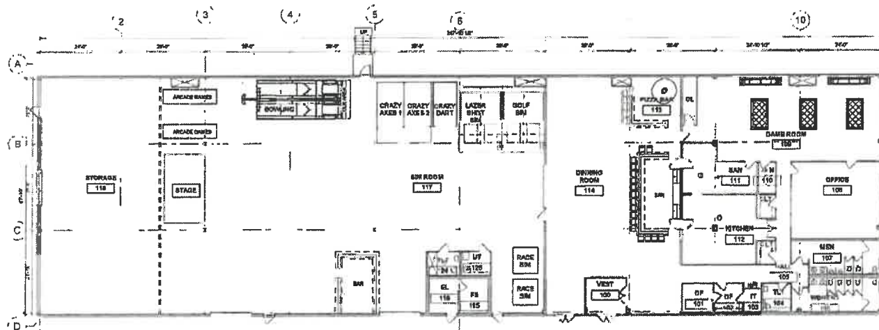
2. FLOOR PLAN 3/8" = 1'-0"
