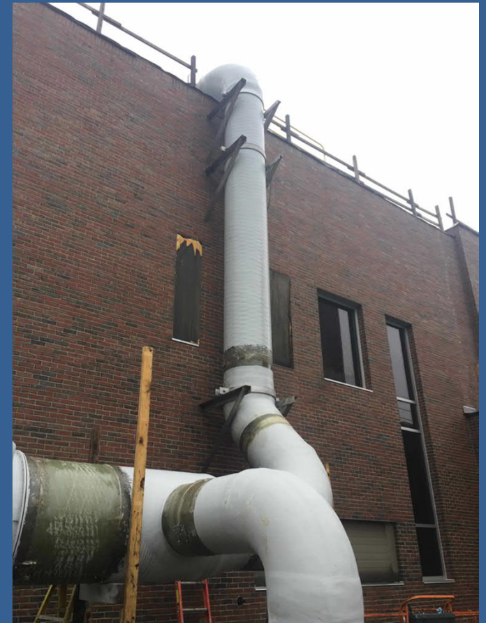
Solids Building
