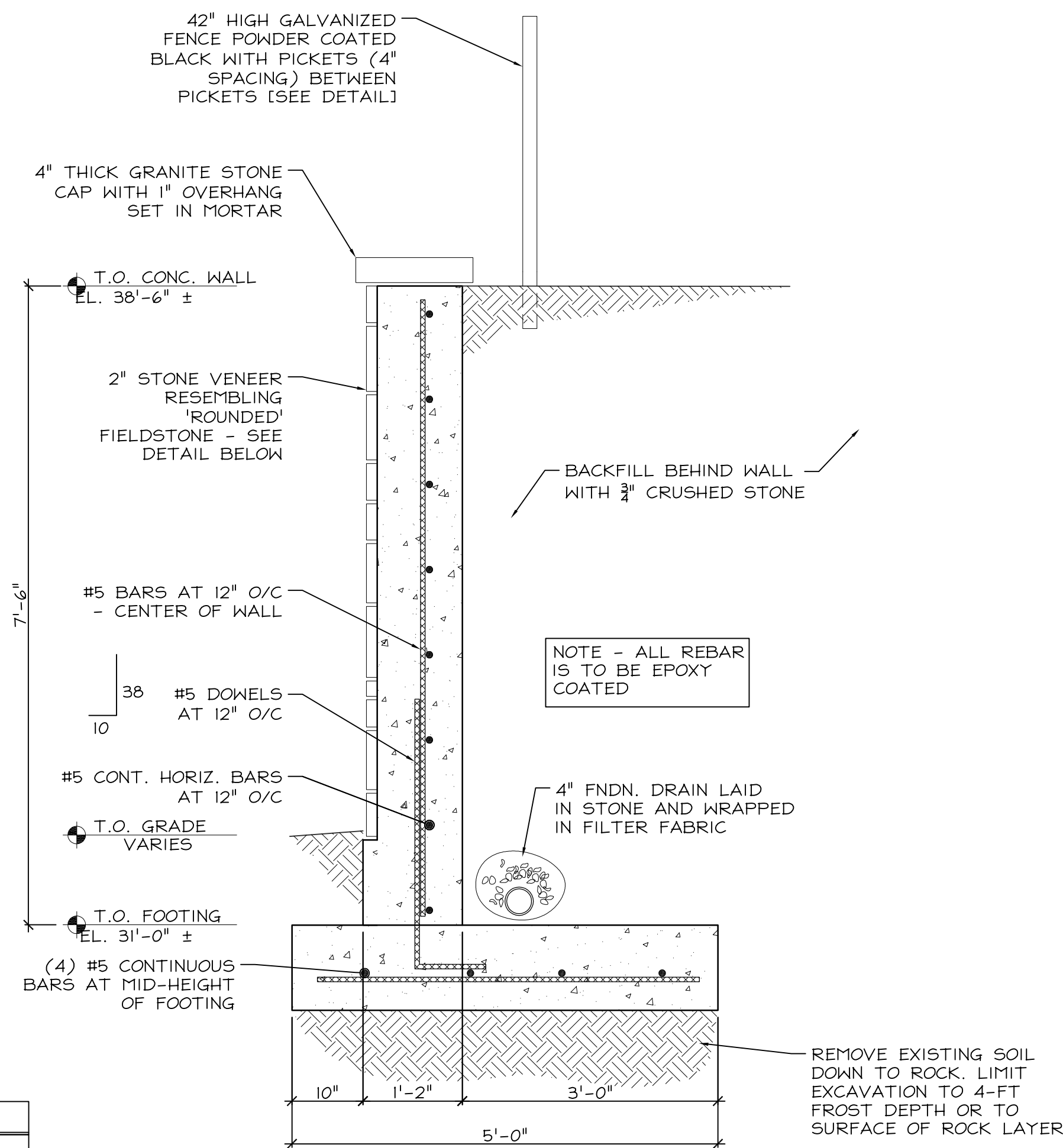
1 RETAINING WALL DETAIL SCALE: 3/4"=1'-0"
