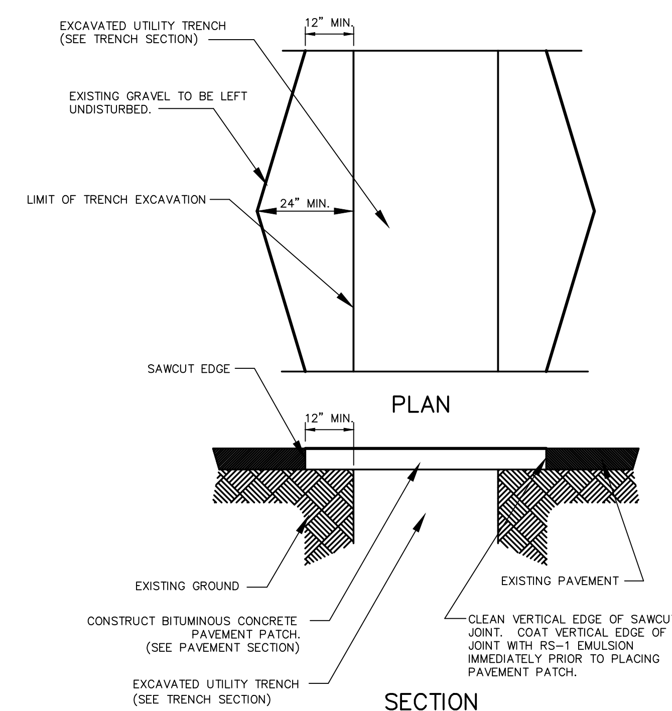
TYPICAL TRENCH PATCH NOT TO SCALE
