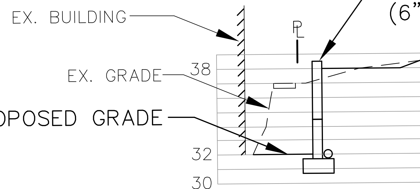
CROSS-SECTION 2
