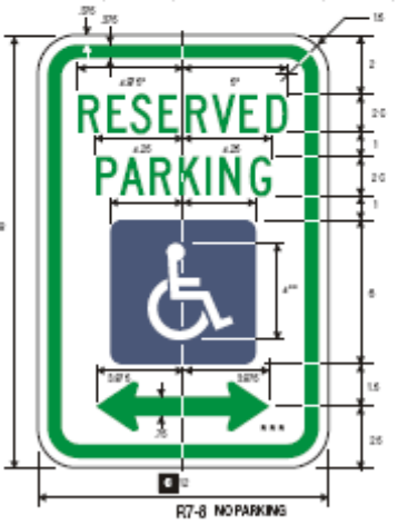
LEGEND - GREEN (RETROREFL) WHITE SYMBOL ON BLUE (RETROREFL) BACKGROUND - WHITE (RETROREFL)
