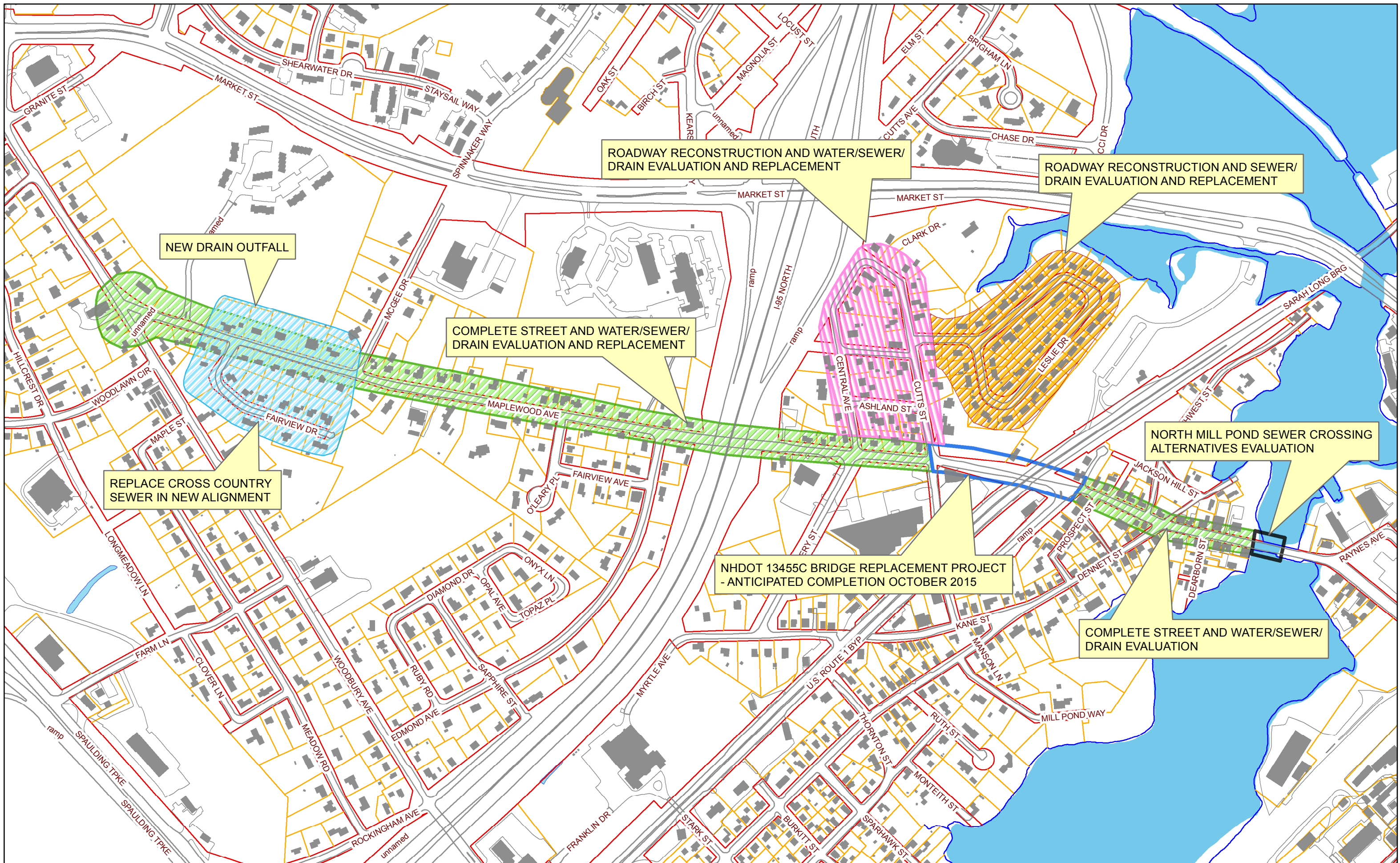
Figure 1 Maplewood Ave Reconstruction
